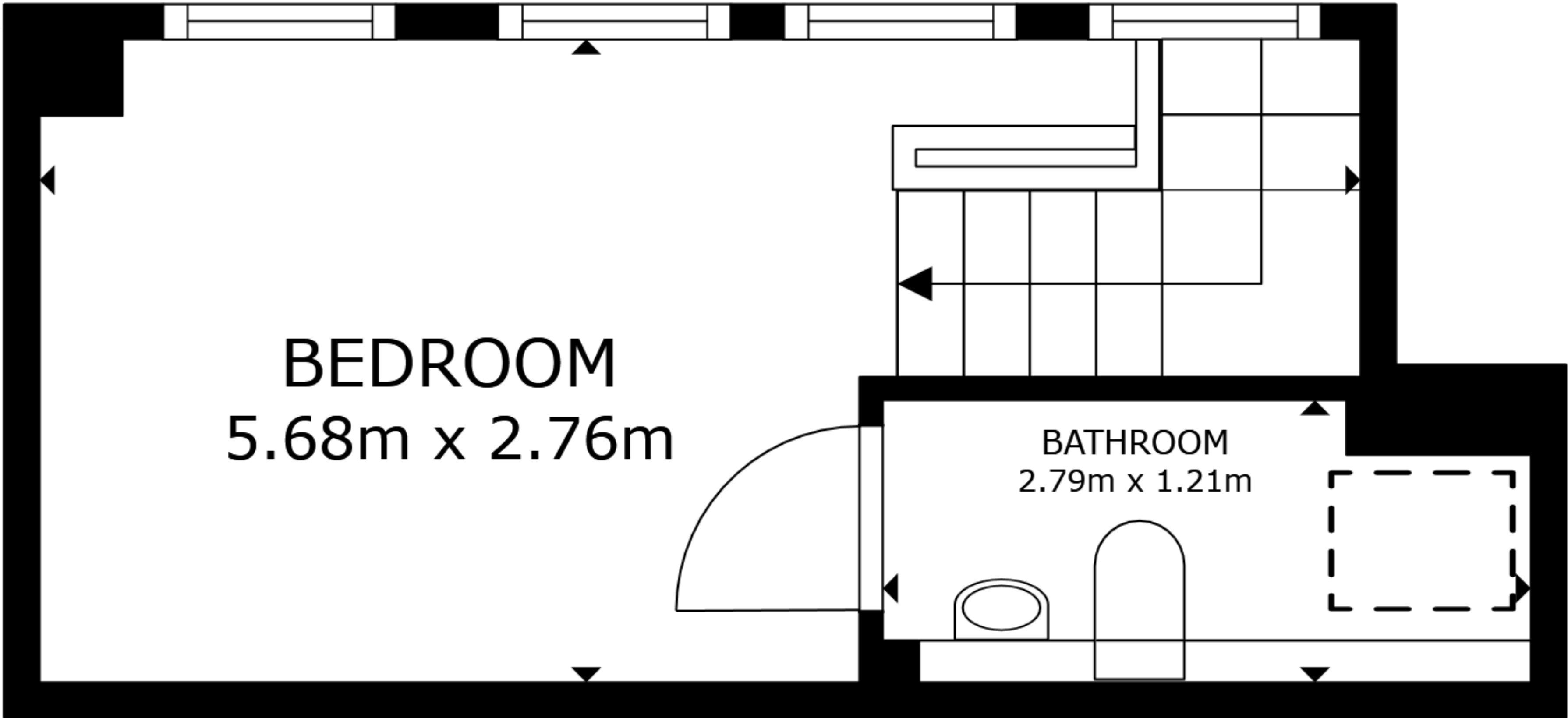
FLOOR 2
